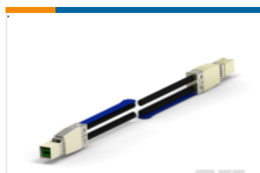
TE Part # 2-2337815-3 MINISAS HD TO MINISAS HD,30AWG, 2M
