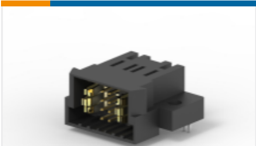
TE Part # 6450834-1 MBXL R/A HDR STR 1P/8S/1P
