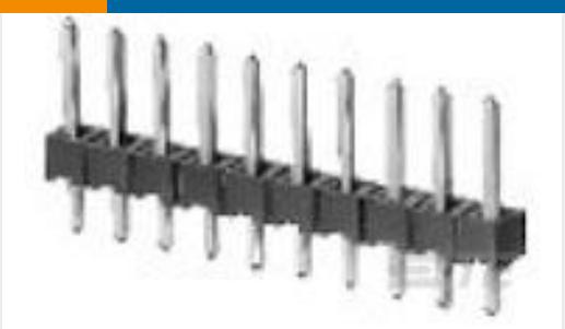
TE Part # 9-146277-0 40 MODII HDR SRST B/A .100CL
