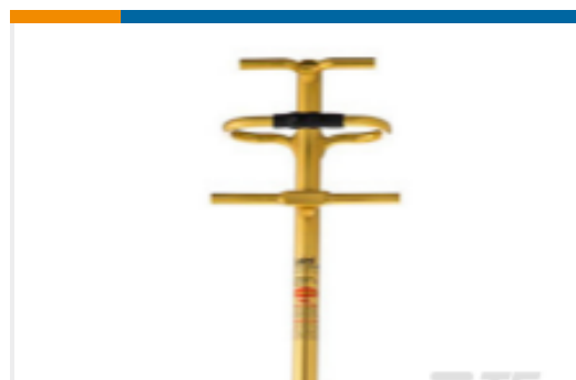
TE Part # YF45018-61NF YAGI,FWG,3,450-490MHZ TB,8.6, FOLDED YAGI
