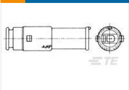
TE Part # 172205-2 ECONOSEAL-J CONN CAP 4P BLACK
