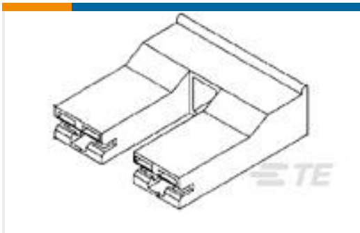
TE Part # 521119-1 PL 250 HOUSING RECEPTACLE NYLON 6/6
