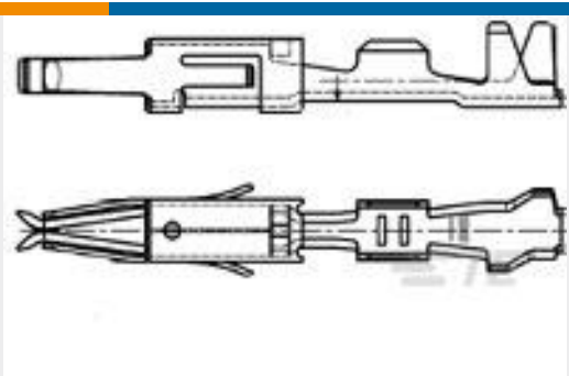
TE Part # 965914-2 MT3 REC 1.6 Contact SRC Sn
