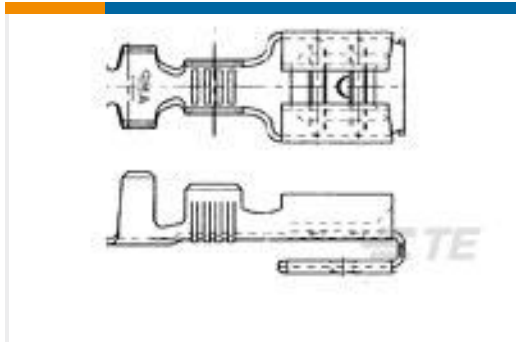
TE Part # 160739-6 250 FASTON, PIGGYBACK REC., 18-14 AWG, PNST
