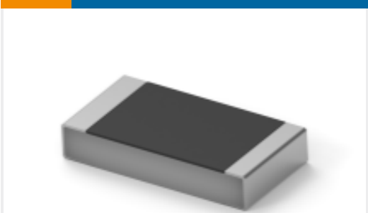
TE Part # 5-2176458-9 CPF 1206 4R02 0.1% 25ppm 1K RL
