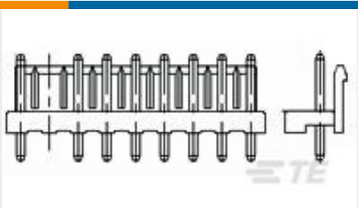
TE Part # 1744109-4 3.96 EP Hdr Assy, 9P, Omitted #8, Blue
