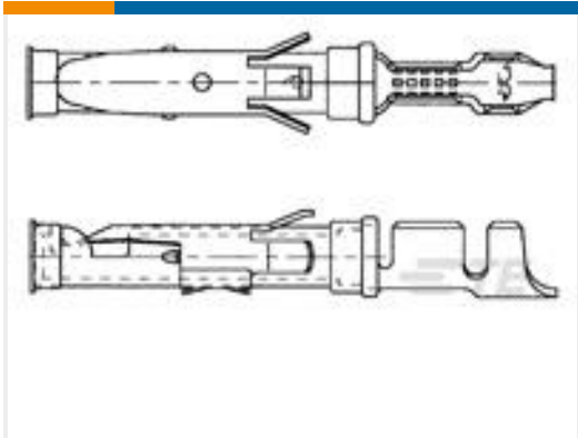
TE Part # 163087-9 062 SOC.ASS. TYP3+
