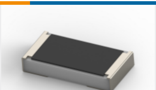
TE Part # 4-2176231-9 SMD Power Resistor: 3 Watt, 1% Tol
