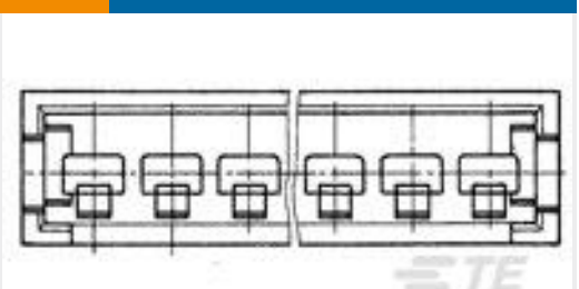
TE Part # 280629 AMPMODU II COSI PIN HSG, SGL ROW, 4 POS.
