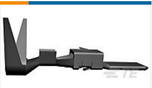
TE Part # 962905-1 TAB AS 4.8x0.8 CONTACT CS SWS Sn TPBR
