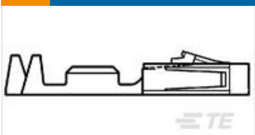
TE Part #104480-8 SHORT POINT RCP CONT LP
