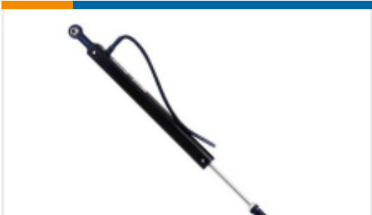
TE Part # CLP-150 LINEAR POT, IP65, 150MM RANGE
