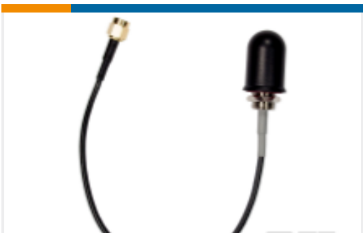
TE Part # L9000168-01 Antenna 2.45/5.8GHz WRT Monopole SMA
