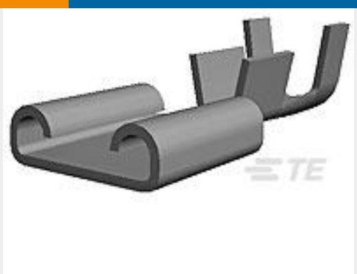
TE Part # 170187-2 250 FASTON,REC.,22-18 AWG,TPBR
