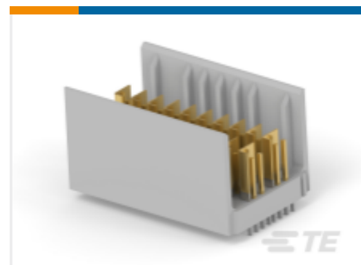
TE Part # 2170328-1 HMZD+, 2PAIRS, 10COLS, VERTICAL, ASSEMBLY
