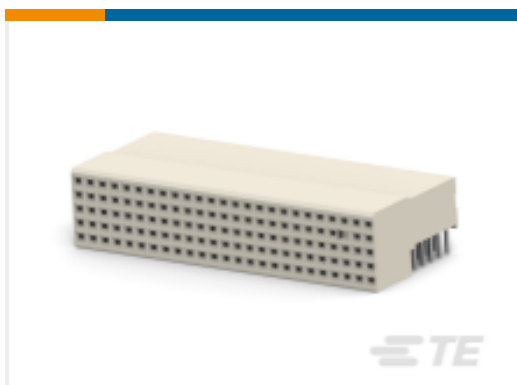
TE Part # 1857990-1 Z-PACK/B F-HDR.125P, EON
