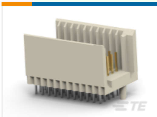
TE Part # 5646529-1 Hard Metric Male Connector: Traditional Backplane, Mezzanine, 2mm
