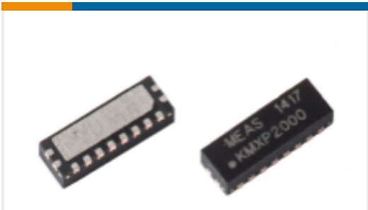
TE Part # G-MR00-050 2MM PITCH AMR POSITION SENSOR KMX
