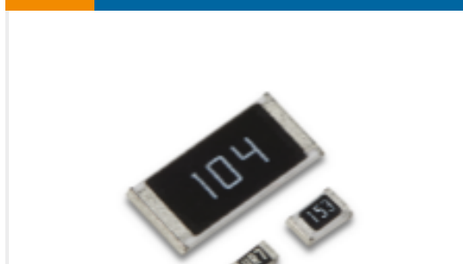
TE Part # 2176341-1 CRGCQ 0805 10R 1%
