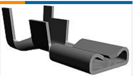
TE Part # 60713-1 FASTON 250 REC 18-14 AWG BR
