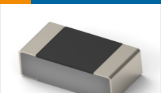
TE Part # 3-2176467-3 TLRP 1206 1.0W R033 1% 100PPM 5K RL
