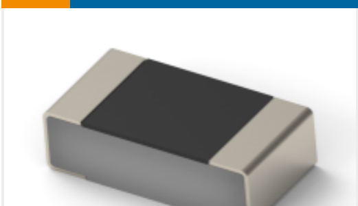
TE Part # 2176467-7 TLRP 1206 1.0W R030 1% 50PPM 5K RL
