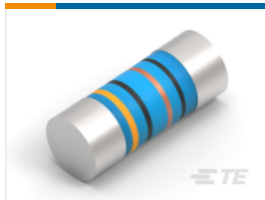
TE Part # 2176316-3 MELF SMA_A 150R 0.1% 15PPM 0207 1W
