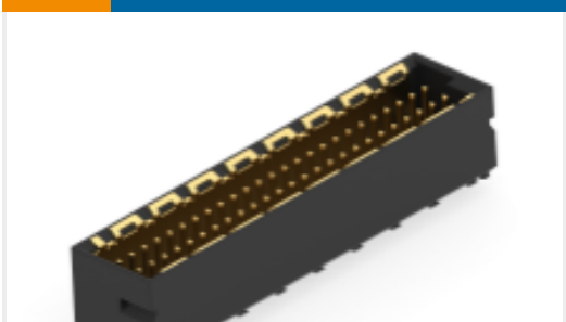
TE Part # 224557-E MSPEED 50 M SMD M2 * AB W 137 094 * * E
