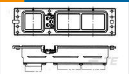
TE Part # 1484613-2 RECP ASSY, SZ 2, ARINC 600
