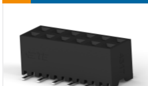
TE Part # 1-2314846-4 14P,2MM,BB,REC,DRVT,SMD,AU.76, TB,W/CP
