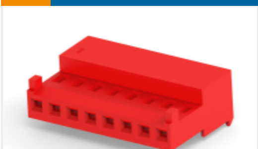
TE Part # 3-644042-8 Nylon Gold Plated Receptacle: 2.54 mm, with Mating Alignment, MTA 100
