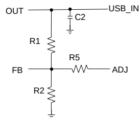
Figure 7: ADJ Configuration
