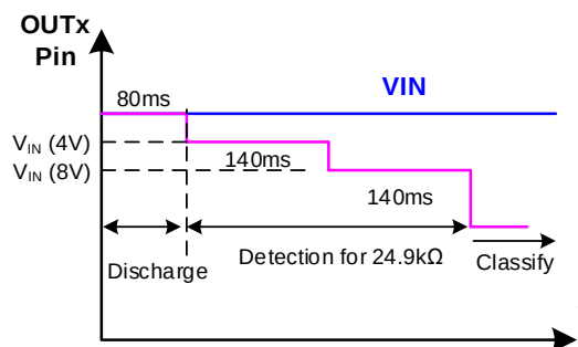
Figure 3: PD Detection Process
