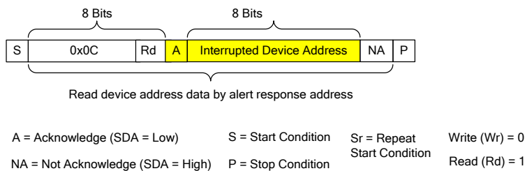
Figure 20: 0x0C Read Example
