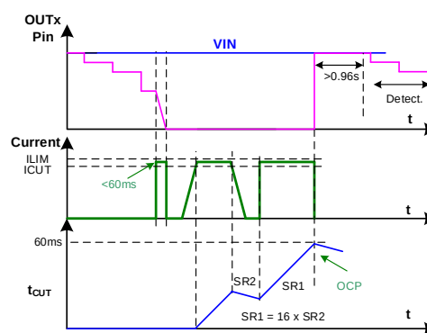
Figure 10: I CUT Over-Current Detection
