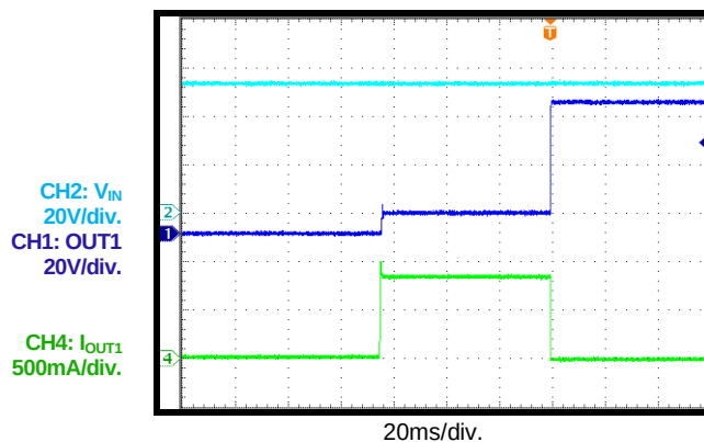
ILIM Triggered
