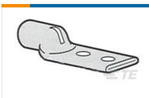
TE Part # 326805 TERMINAL,AMPPOWER 300MCM 3/8
