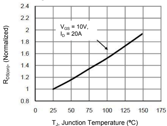
Figure 7. Drain-Source On-Resistance
