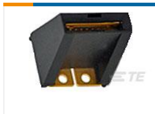
TE Part # 1926671-1 CROWN CLIP SENIOR POWER SKT GOLD PLATING
