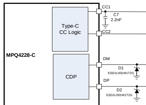
Figure 13: Recommended I/O Pins ESD Enhancing
