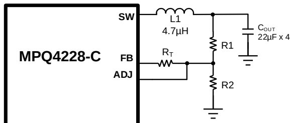
Figure 6: Line Drop Compensation
