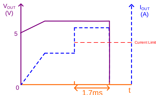
Figure 7: Over-Current Limit
