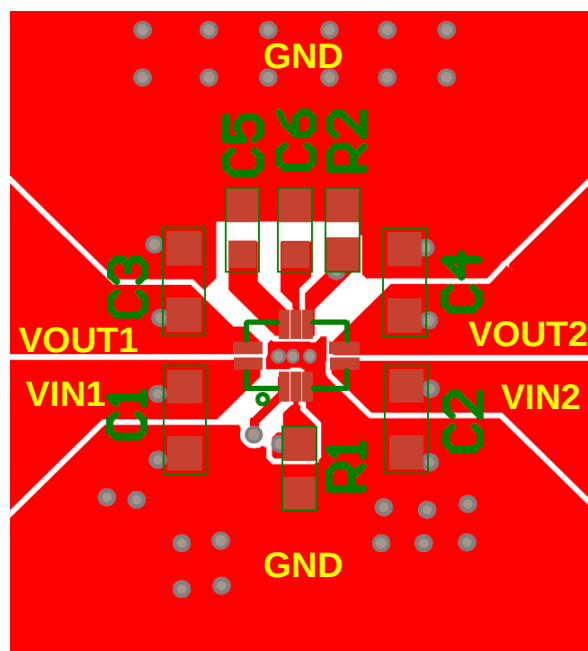
Figure 2: Recommended PCB Layout
