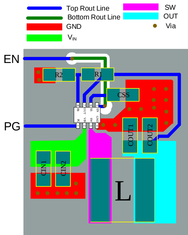
Figure 8: Recommended PCB Layout
