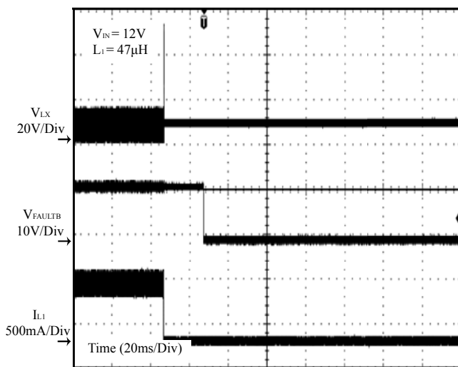
Figure 24 Diode Open
