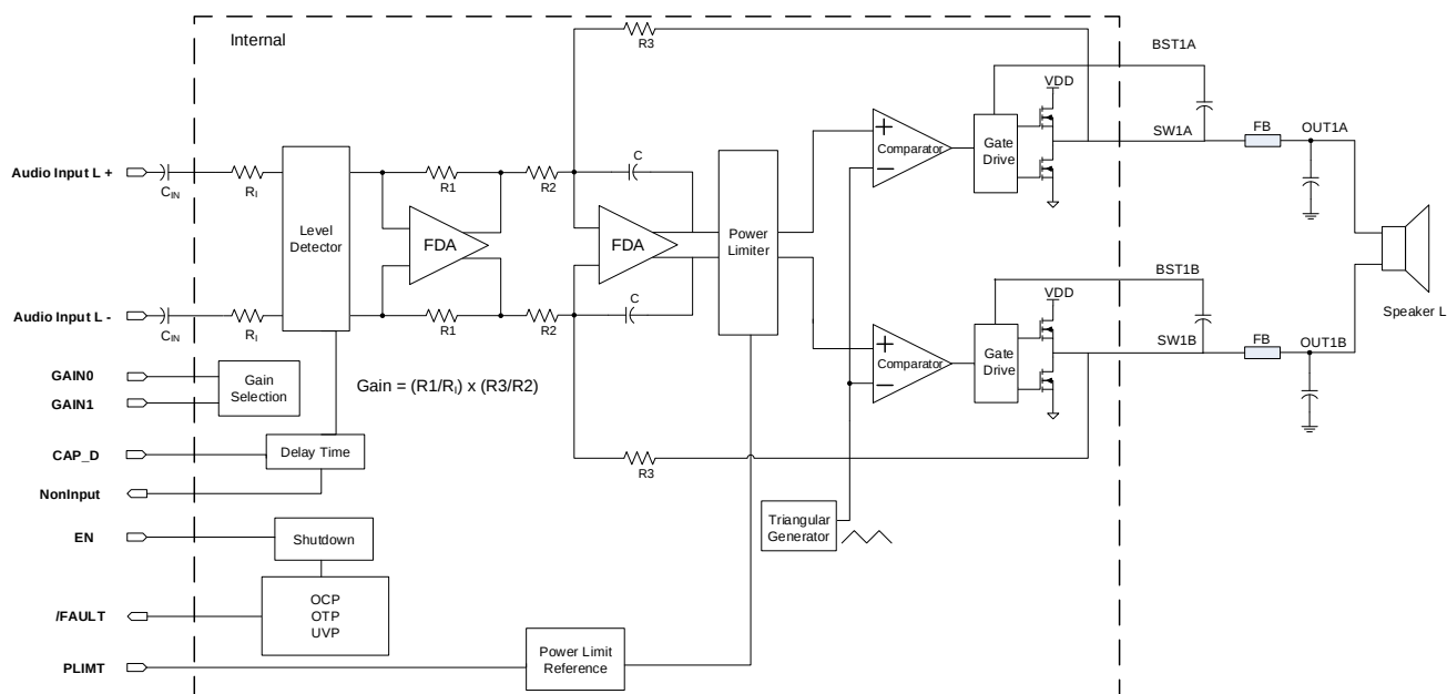
Figure 1: Functional Block Diagram (One Channel)
