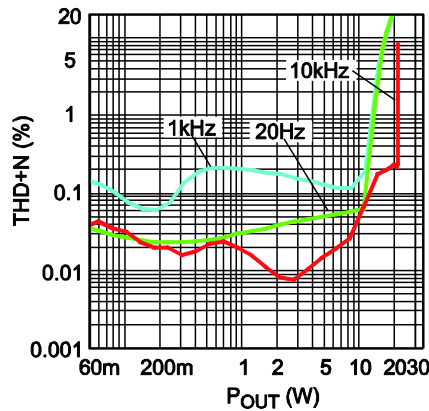
THD+N vs. POUT 12V, 4Ω + 33μH
