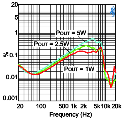
THD+N vs. Frequency 12V, 4Ω + 33μH
