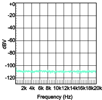
FFT Noise Floor Test 12V, 4Ω + 33μH
