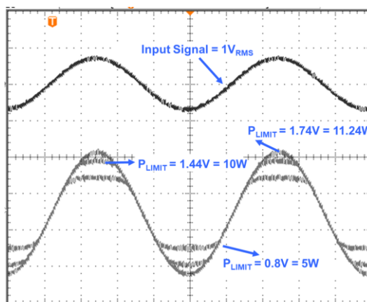
Figure 4: PLIMIT Circuit Operation
