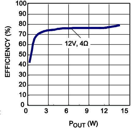
Efficiency vs. POUT 4Ω + 33μH
