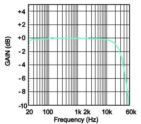
Frequency Response 12V, 4Ω + 33μH, 1W
