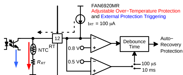
Figure 44. Adjustable Over-Temperature Protection
