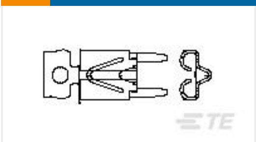
TE Part # 1217080-1 FASTON 205/250 PCB MOUNTED TPBR
