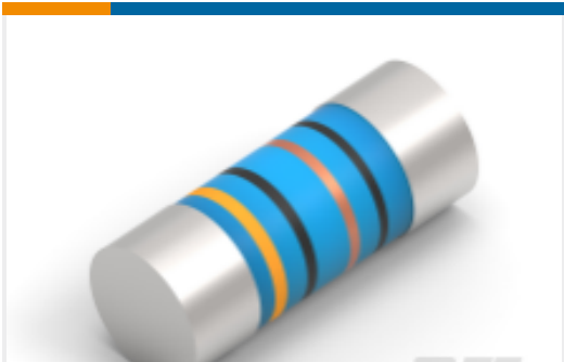
TE Part # 1-2176315-6 MELF SMA_A 1K8 0.1% 15PPM 0204 0.4W
