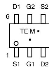
SOT-363 CASE 419B STYLE 26
