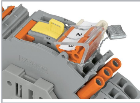
A lock-out seal can be used on the disconnect link in operating position I when combined with an end and separator plate (Item No. 2007-8893 or Item No. 2007-8894).
