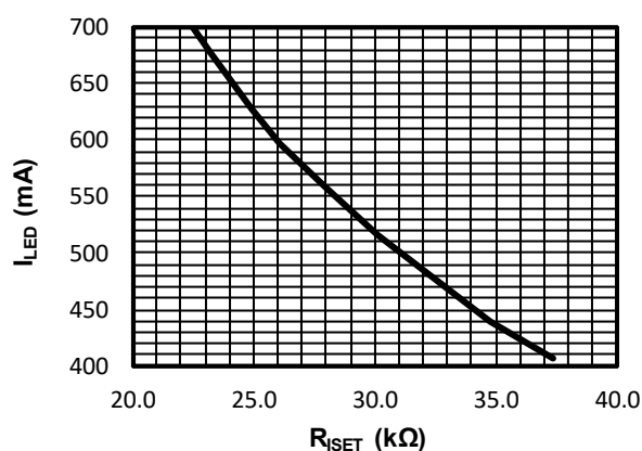
Figure 1: I_{LED} vs. R_{ISET} when I_{LED} \leq 700mA in Buck-Boost Mode
