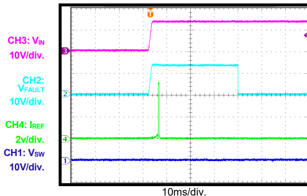
I_{REF} Open before VIN Start-Up
