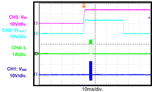
Mode Detect Wrong at VIN Start-Up
