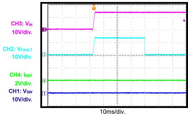
I_{REF} Short before VIN Start-Up
