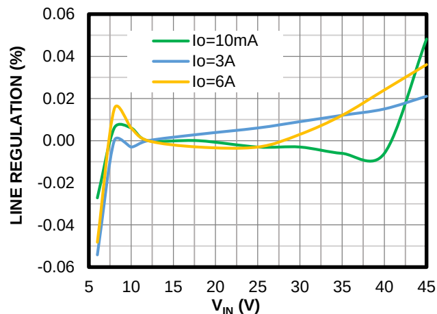
Line Regulation
