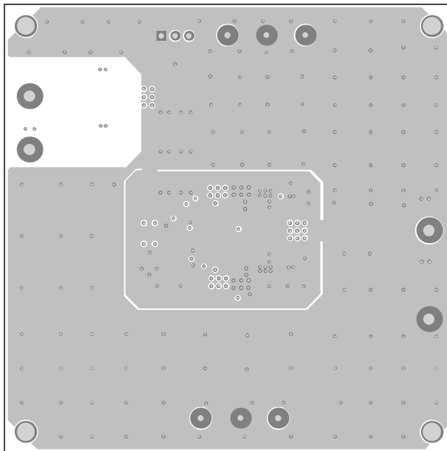
Figure 5: Mid-Layer 1
