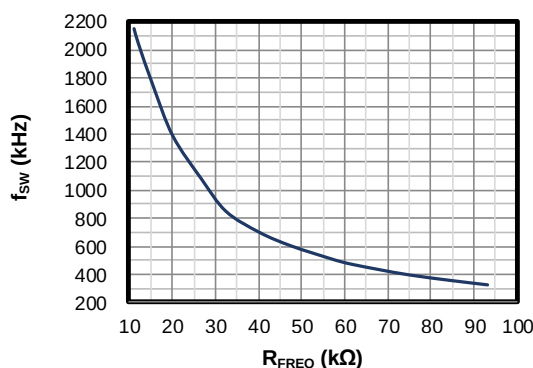
Figure 1: f_{SW} vs. R_{FREQ}
