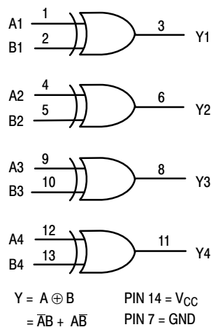
Figure 1. Logic Diagram
