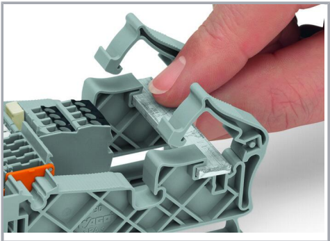
Place the busbar in the carrier holder.
