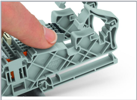
Snapping the busbar carrier onto DIN-35 rail.
