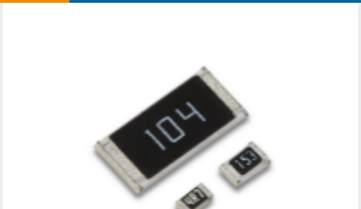
TE Part # 2-2176337-0 CRGCQ 0402 390R 1%
