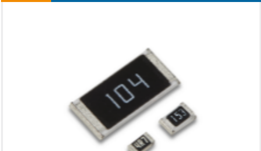
TE Part # 1-2176337-6 CRGCQ 0402 180R 1%
