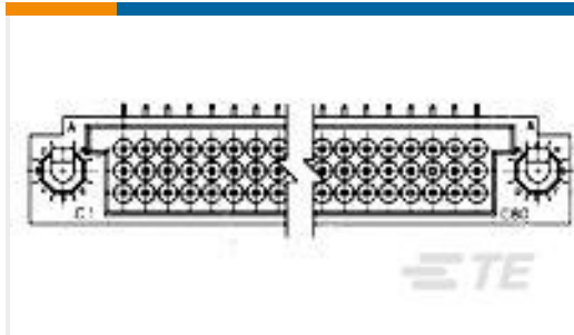
TE Part # 448007-1 3 ROW BOX PIN 180 POS R/A
