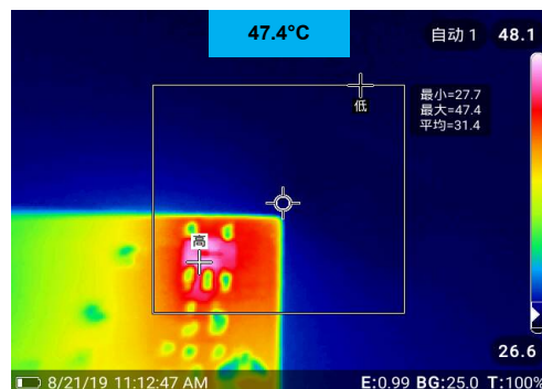
Thermal V_{IN}=265V_{AC}
