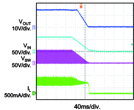
Power Off I_{OUT} = 300mA
