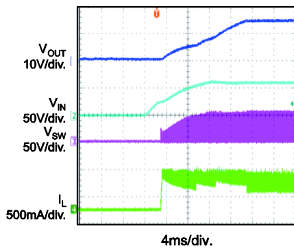
Power On I_{OUT} = 300mA
