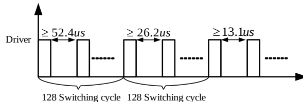
Figure 4: t_{\text{minoff}} at Start-Up
