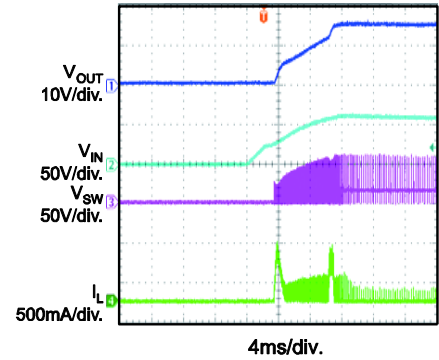
Power On I_{OUT} = 5mA
