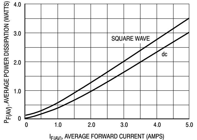
Figure 4. Power Dissipation
